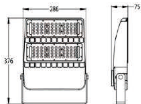
FL80W-100W/E FL80WHV-100WHV/E
