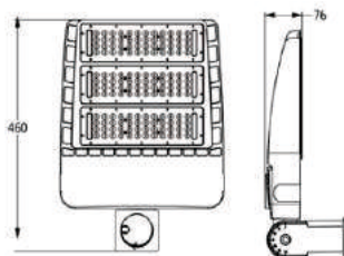
FL120W-180W/A FL120WHV-180WHV/A
