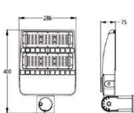
FL80W-100W/A FL80WHV-100WHV/A
