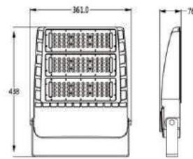
FL120W-180W/E FL120WHV-180WHV/E
