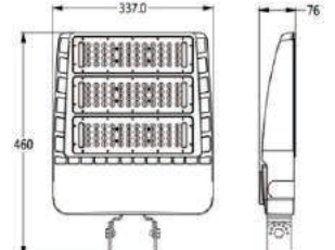
FL120W-180W/C FL120WHV-180WHV/C
